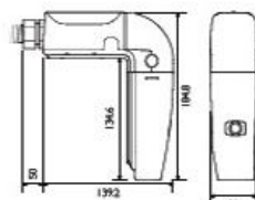
Vertical 90 Degree Print Head Installation Dimensions
