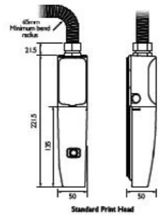
Standard Print Head
