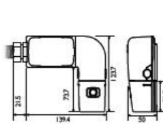
Horizontal 90 Degree Pinpoint Print head
