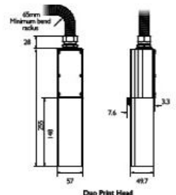
Duo Print Head
