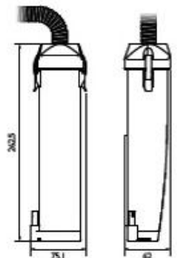
Heavy Duty Print Head
