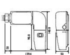
Horizontal 90 Degree Print Head Installation Dimensions
